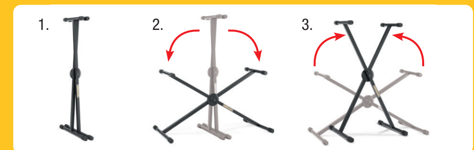
Simply set the stand by: 1st, closing the stand entirely, 2nd opening it all the way to the lowest level and 3rd raising it to the desired height. The EZ-LOK System automatically locks stand into one of five height settings. No more fussing with screws! Repeat above operation 1-3 to reset the height.
